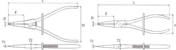
SS-175LK・SS-230LK
